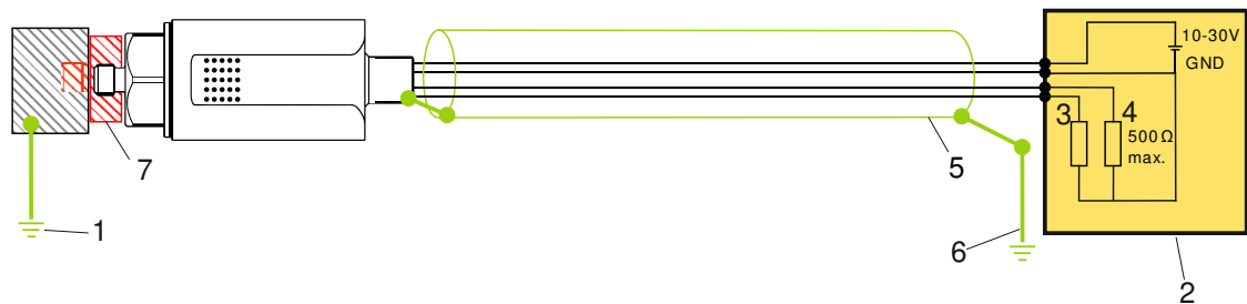
Fig. 11: Alternative earthing concept
